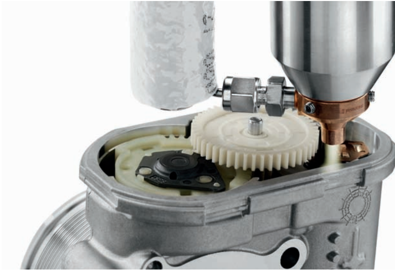
Fig. 4: Applying «PlasmaPlus» coating to a die-cast aluminum prior to bonding: This inline technology can be used to generate product-specific multifunctional coatings and deposit them in precisely defined areas in a matter of seconds.
