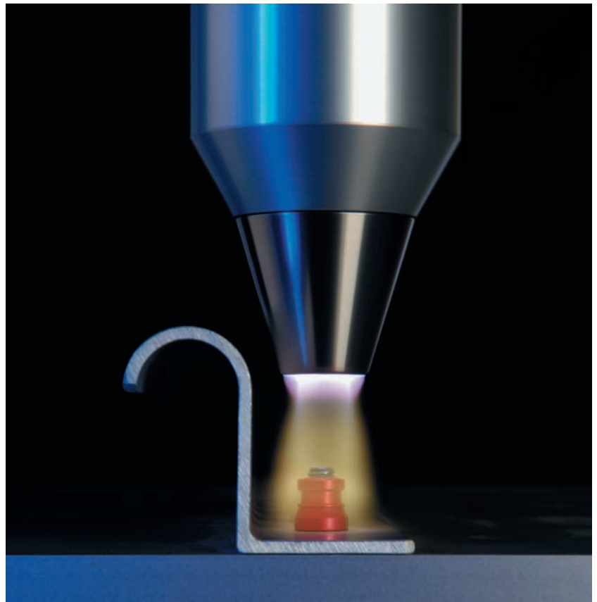
Fig. 6: Aircraft manufacturing: The edges of the tiny rivets are susceptible to damage and corrosion. With contact-free plasma, they can be pretreated without risk of damage.
